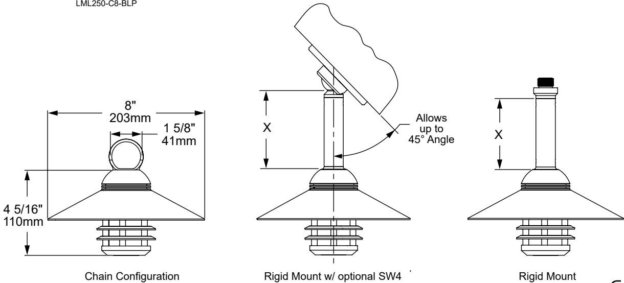
Chain Configuration
