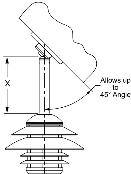
Rigid Mount w/ optional SW4
