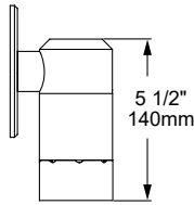
HWM16-1 [90°] Straight Shield
