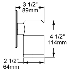
HWM16-1 [FS] Flush Shield
