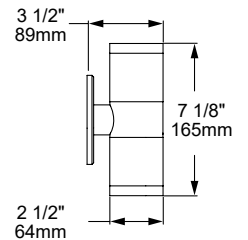
HWM16-2 [FS] Flush Shields
