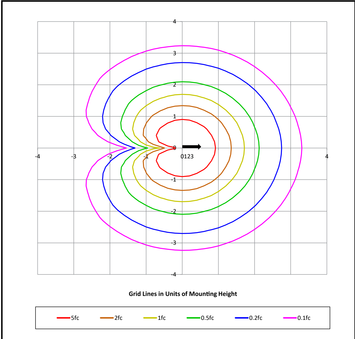
Mounting Height - 2 Feet
